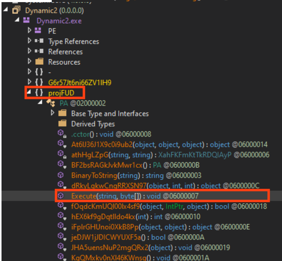
Injector's decompiled code.
