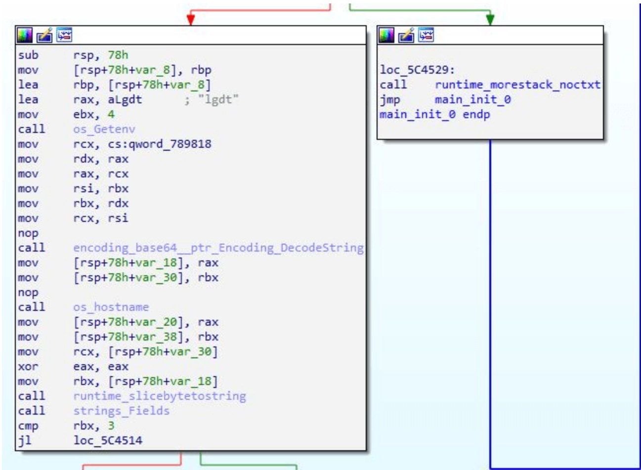
Figure 10. Routine that decrypts environment variables and uses them as configuration data In the attack case in Korea covered above, three arguments are found after decoding with Base64. These are the C2 server URL, port number, and wait time.
