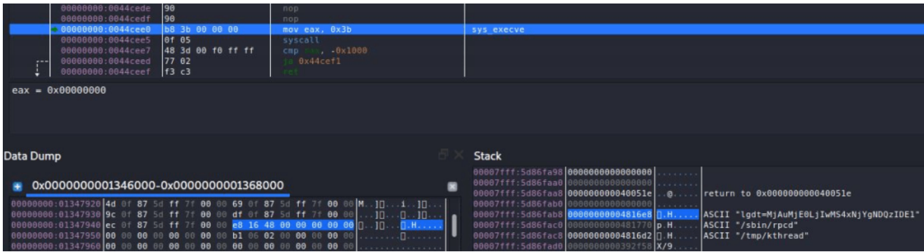
Figure 9. lgdt environment variable transmitted upon execution
