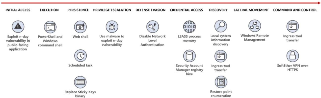
Figure 1. Flax Typhoon attack chain
