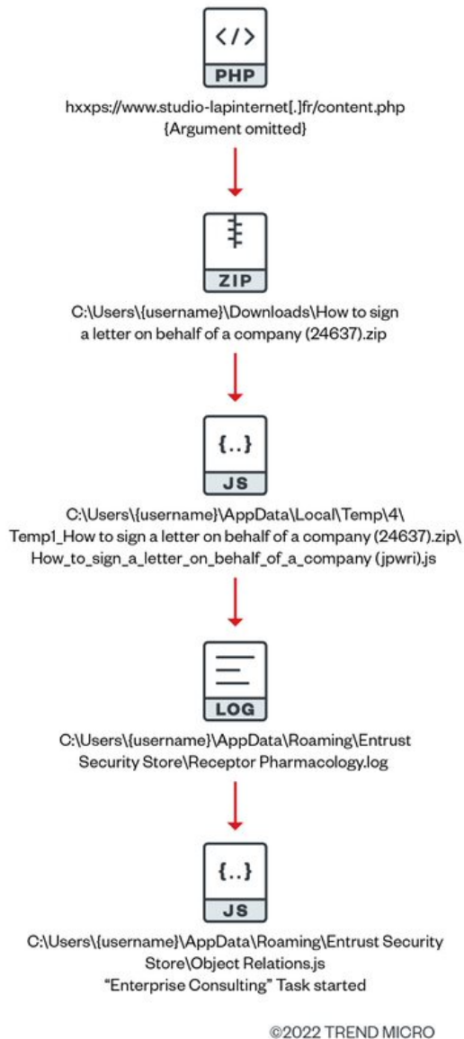
Figure 4. Chain of malicious files with file names and Gootkit loader features
