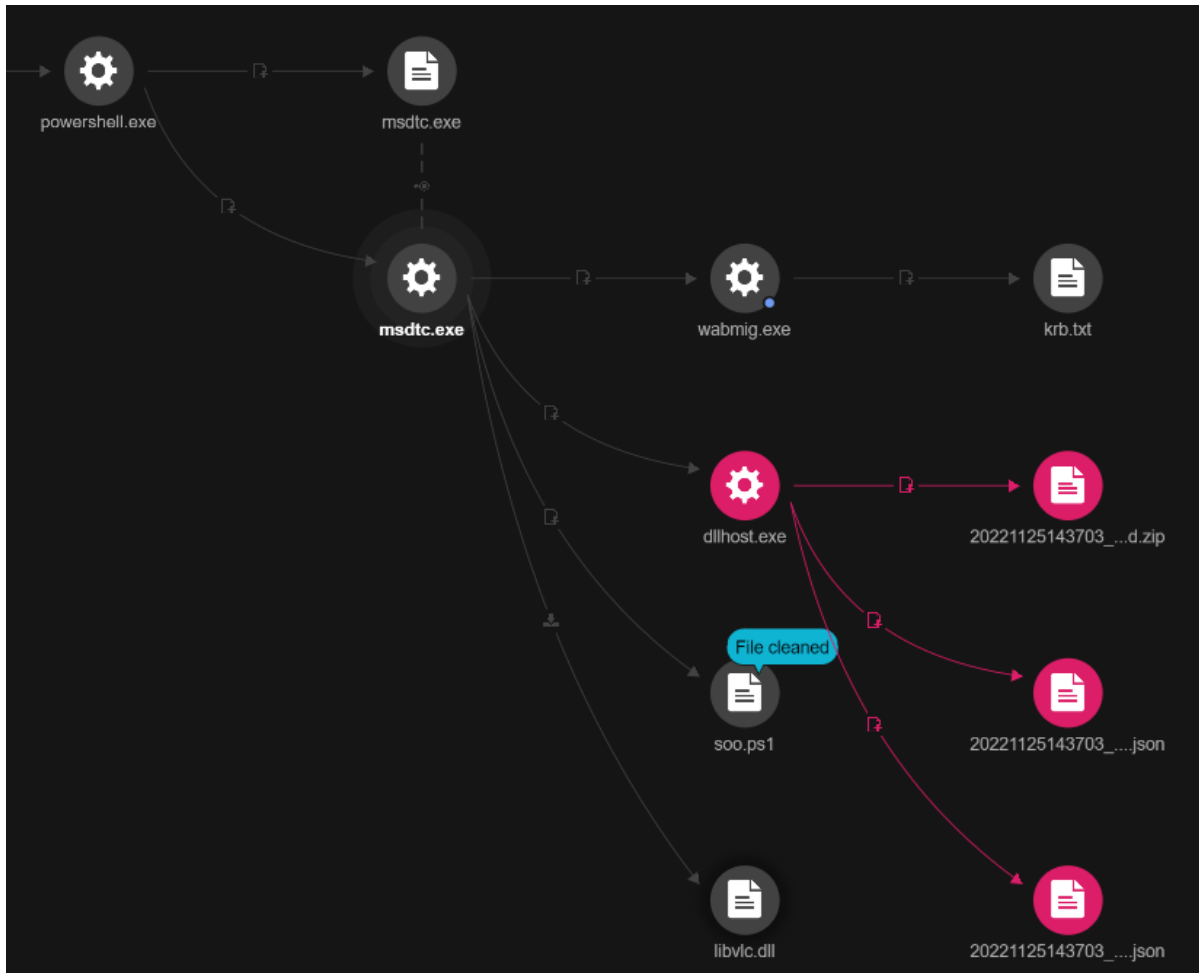
Figure 15. Process chain showing activities related to msdtc.exe
