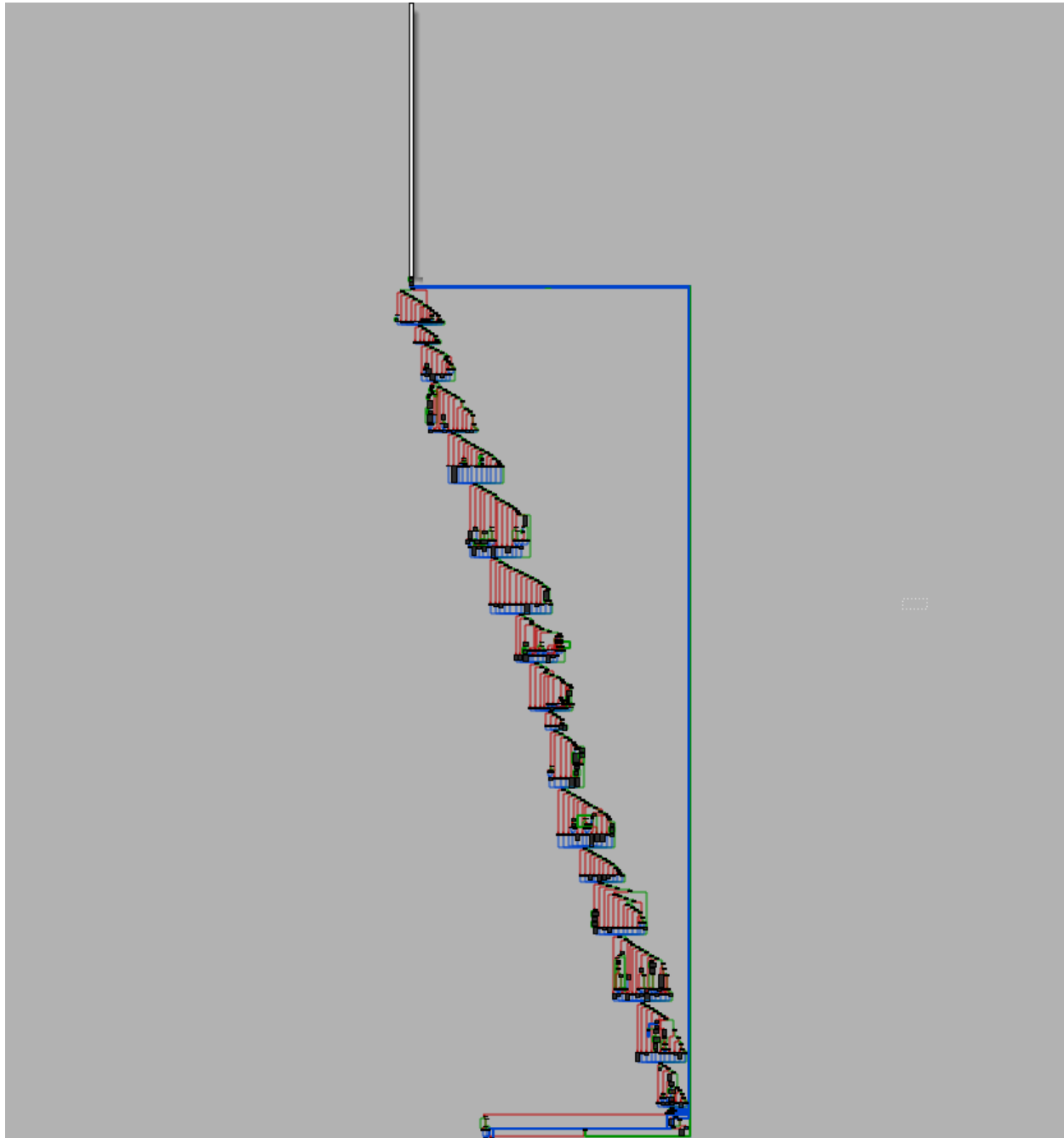
Control flow graph of a function obfuscated using control flow flattening
