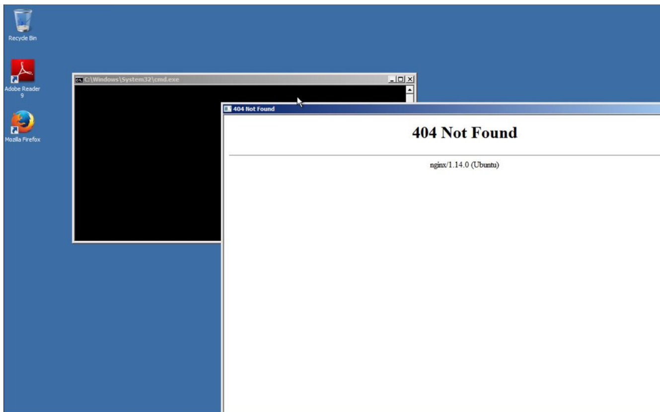
Image 32. Screenshot of the error receiving the second stage of the payload.
