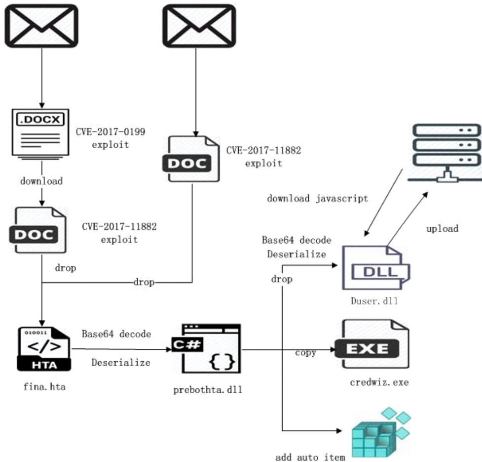
Image 33. Fragment of Kill Chain taken from https://mp.weixin.qq.com/s/Kkta59k7r81uIBjJvE9pCw
