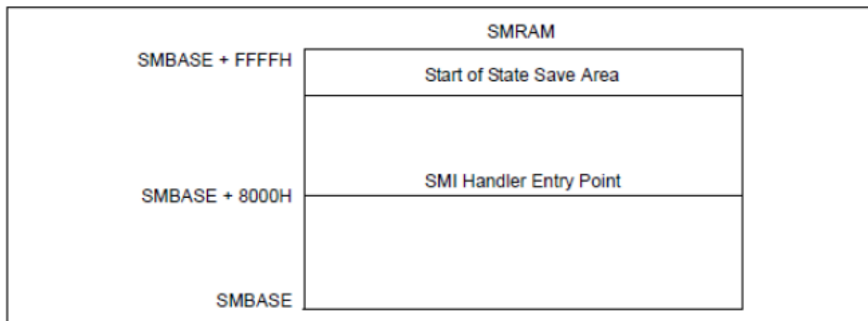
Figure 34-1. SMRAM Usage
