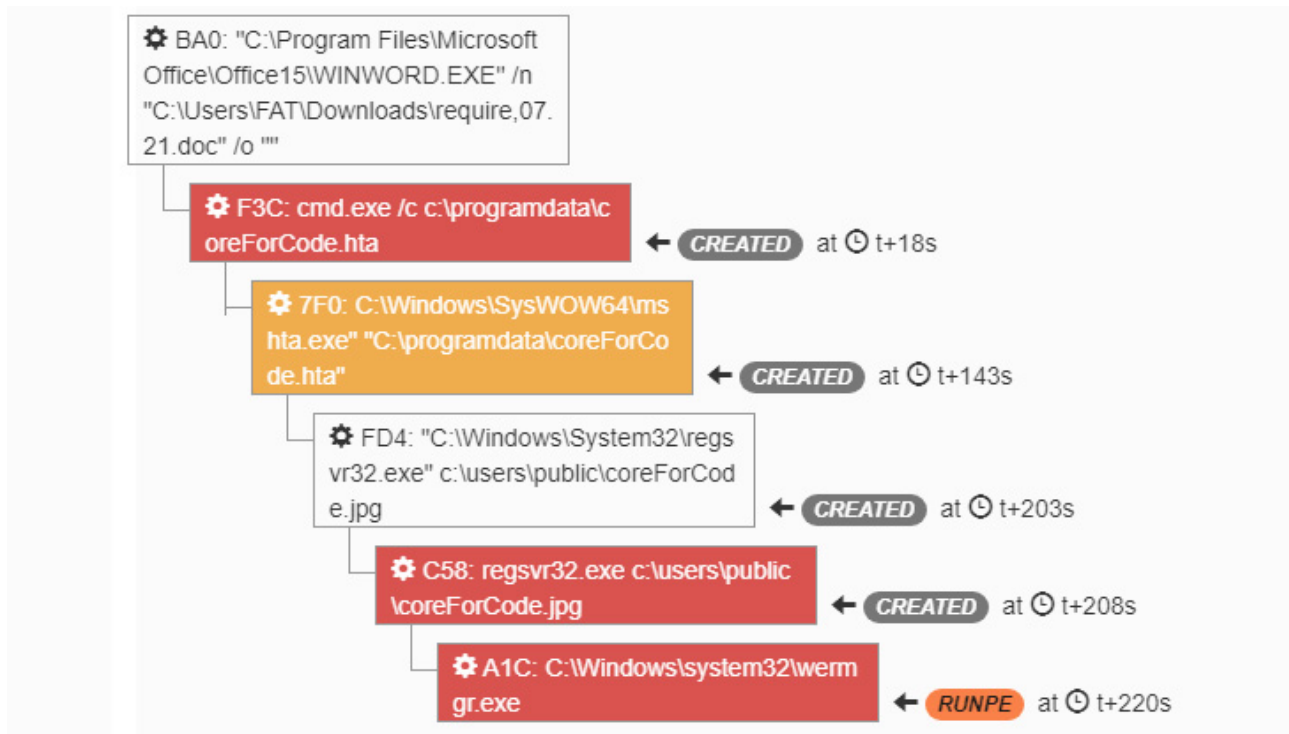
Figure 1 - Trickbot execution in the sandbox
