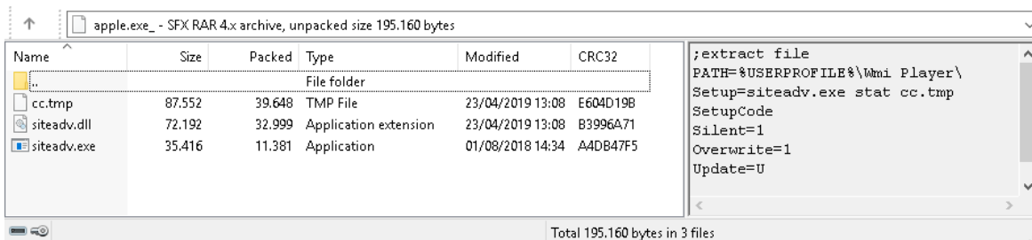
Figure 3. Contents of the apple.exe archive
