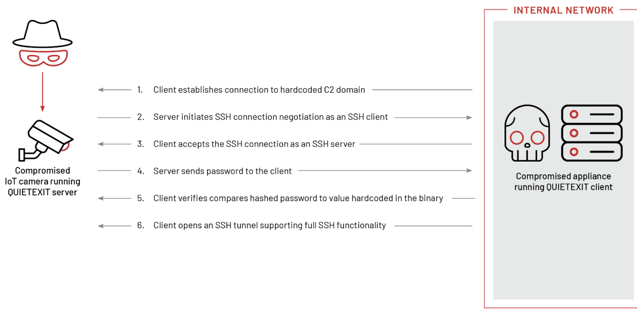
Figure 1: How QUIETEXIT works with IoT devices
