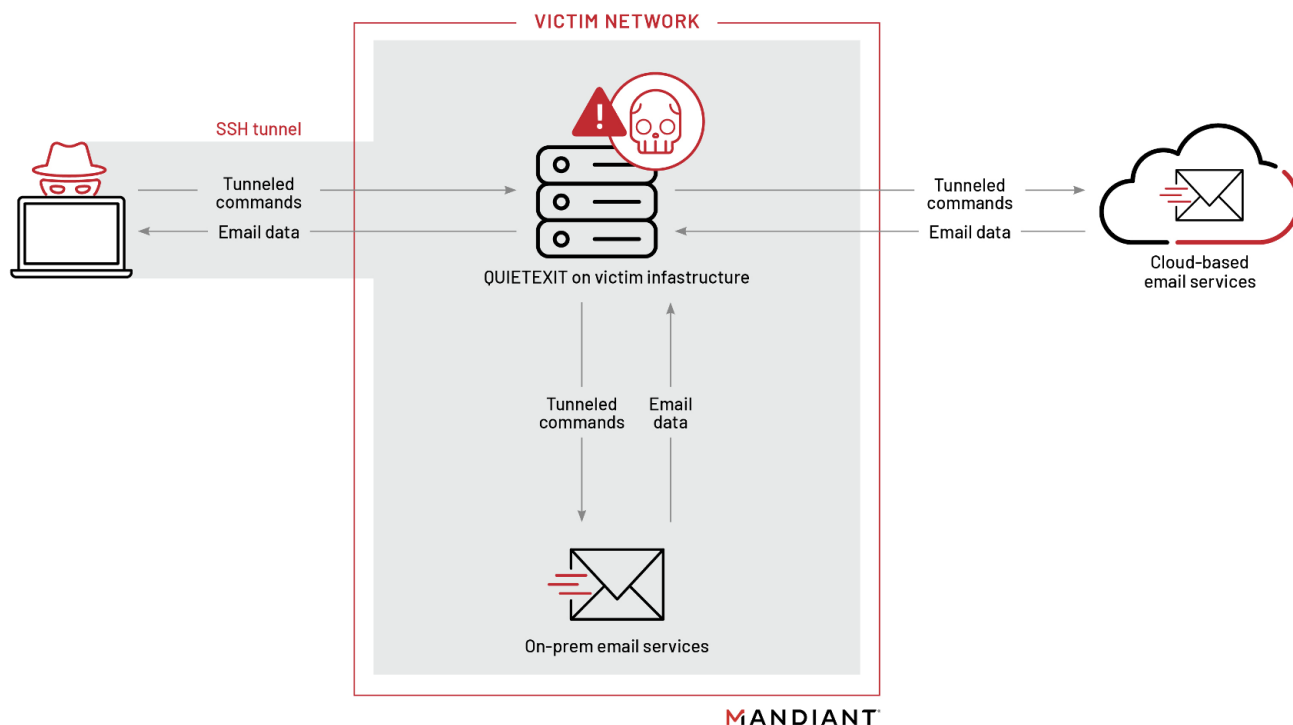
Figure 2: Tunneling through QUIETEXIT
