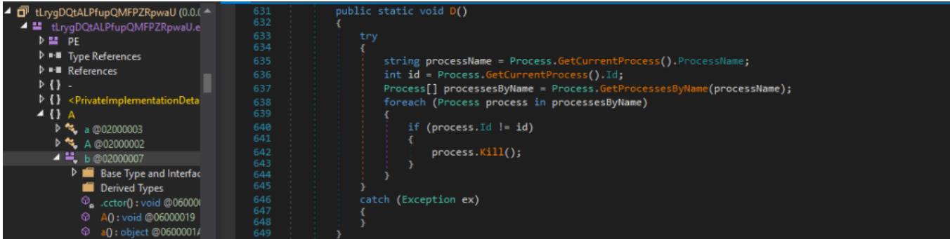
Figure 8: AgentTesla Payload
