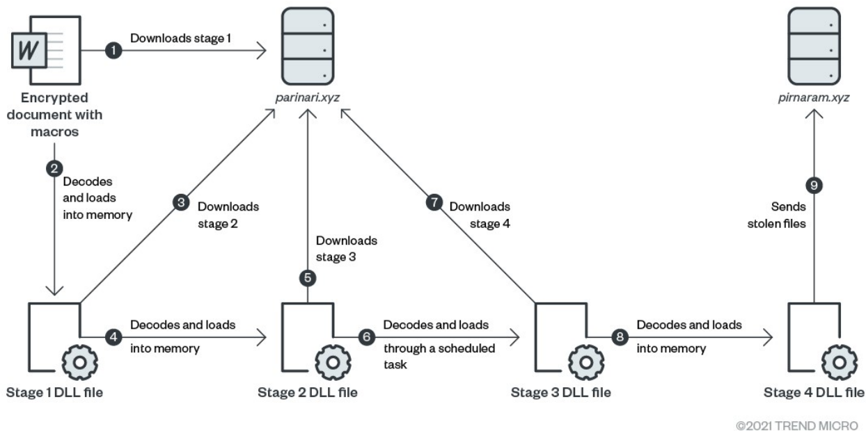
Figure 3. File stealer loading scheme
