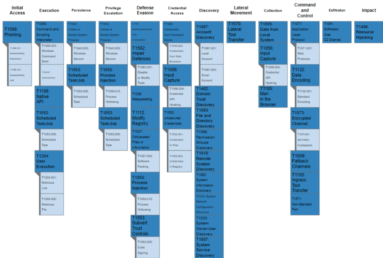
Figure 1: MITRE ATT&CK enterprise techniques used by TrickBot
