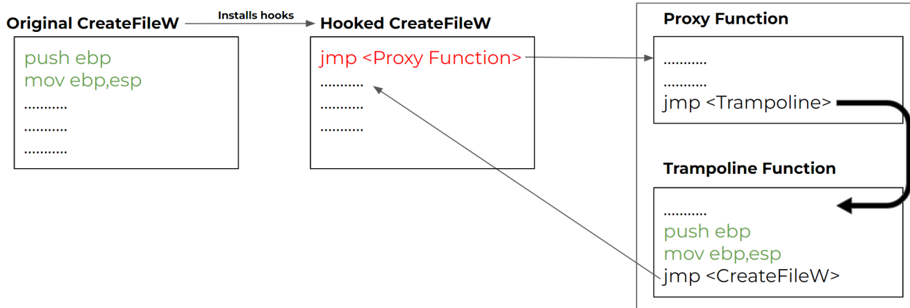
Figure 3. Inline Hooking Example
