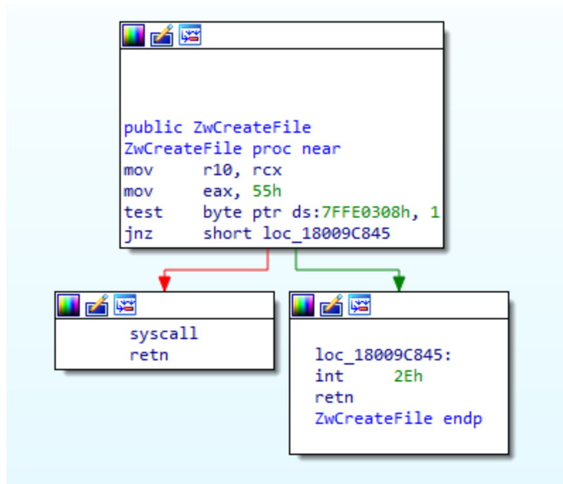
Figure 2. System call stub for ZwCreateFile in ntdll
