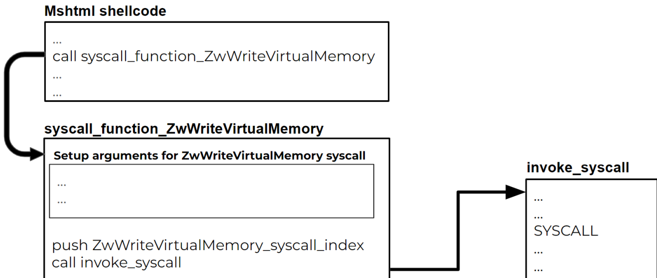
Figure 7. Lumma Stealer direct syscall invocation chart
