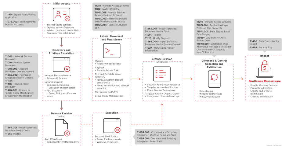
Figure 3. The Gentlemen ransomware attack chain
