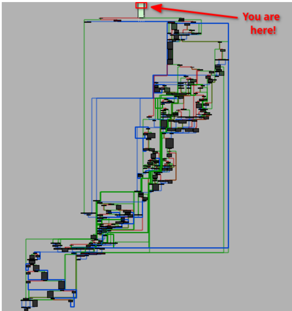
KrustyLoader main routine
