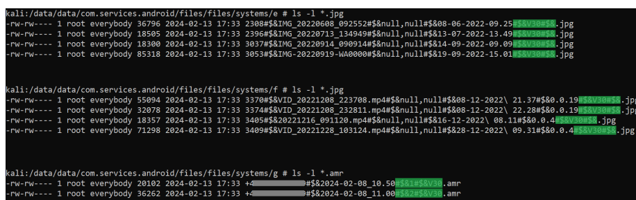
Figure 15. Filenames of multimedia data exfiltrated from device (highlighted is the embedded malware version number)
