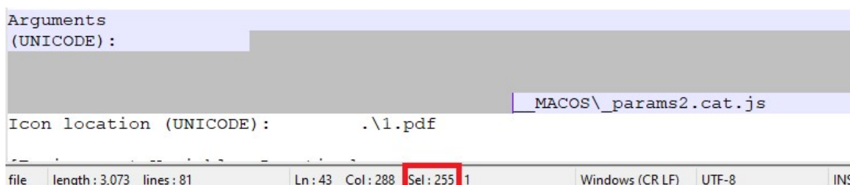
Figure 4. 255 space characters were used before the actual argument value.
