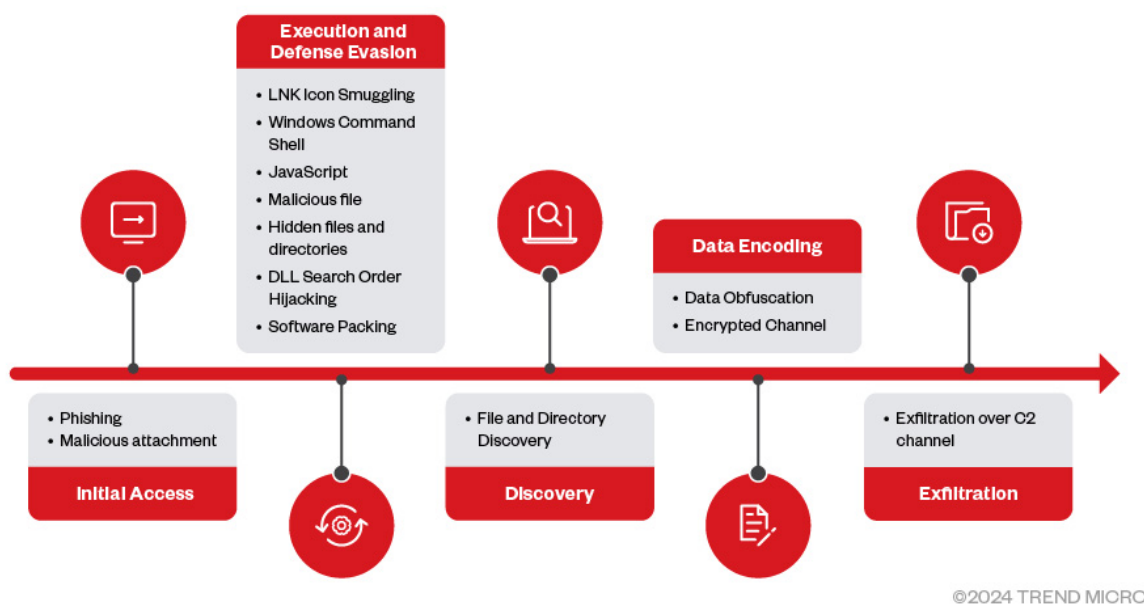
Figure 1. The infection chain used in the campaign download
