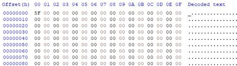
Figure 7. File overwritten before being deleted
