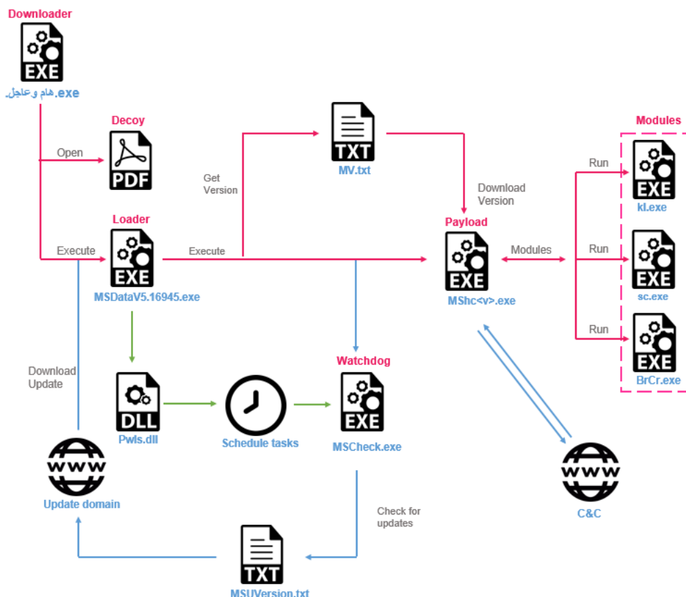
Figure 1 – Infection flow for Stealth Soldier (Version 9).
