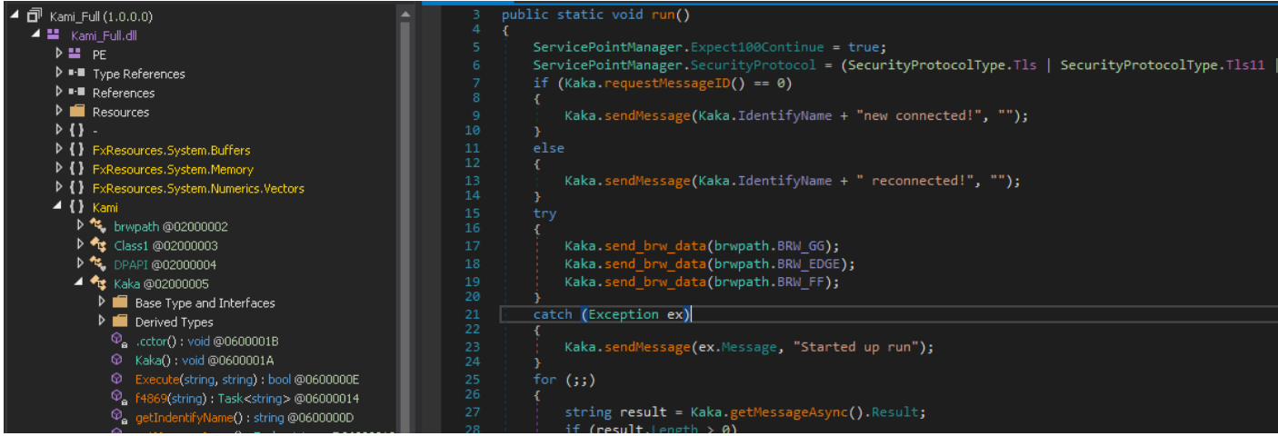
Figure 13: Screenshot detailing decompiled executable that contains KamiKakaBot
