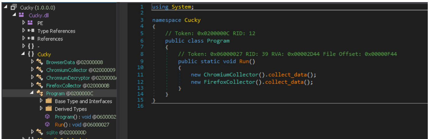
Figure 12: Screenshot of decompiled Cucky stealer
