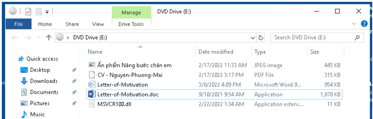
Figure 4: Screenshot detailing the five files contained in one ISO image seen by Group-IB. Note that the .doc and .dll files are in hidden view.
