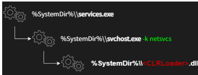
Figure 2. Process tree running CLRLoader
