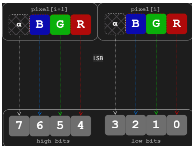
Figure 5. Byte reconstruction from 2 pixels
