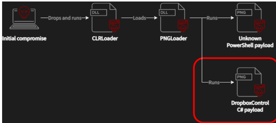
Figure 13. Extended compromise chain
