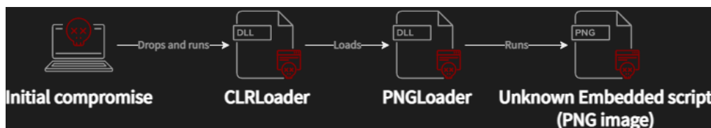
Figure 1. Worok compromise chain
