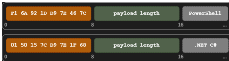
Figure 6. Data structure embedded in PNG bitmap
