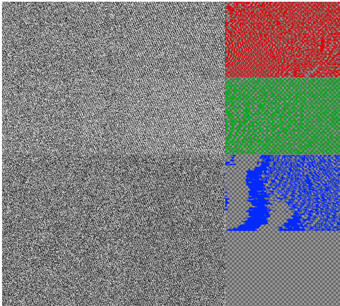
Figure 11. Zero (LSB) bit-planes channels with embedded data
