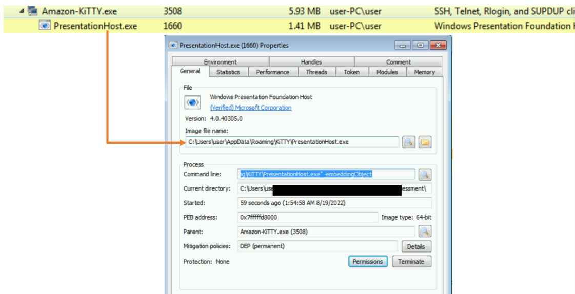
Figure 4. KiTTY – DLL search order hijacking
