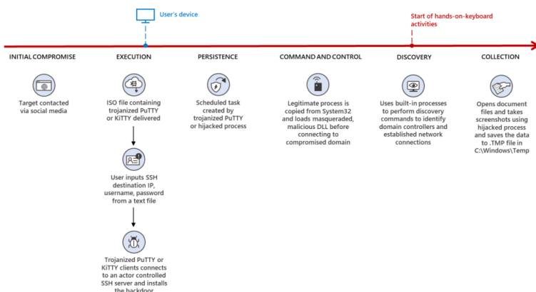
Figure 1. Attack flow diagram for recent ZINC campaign
