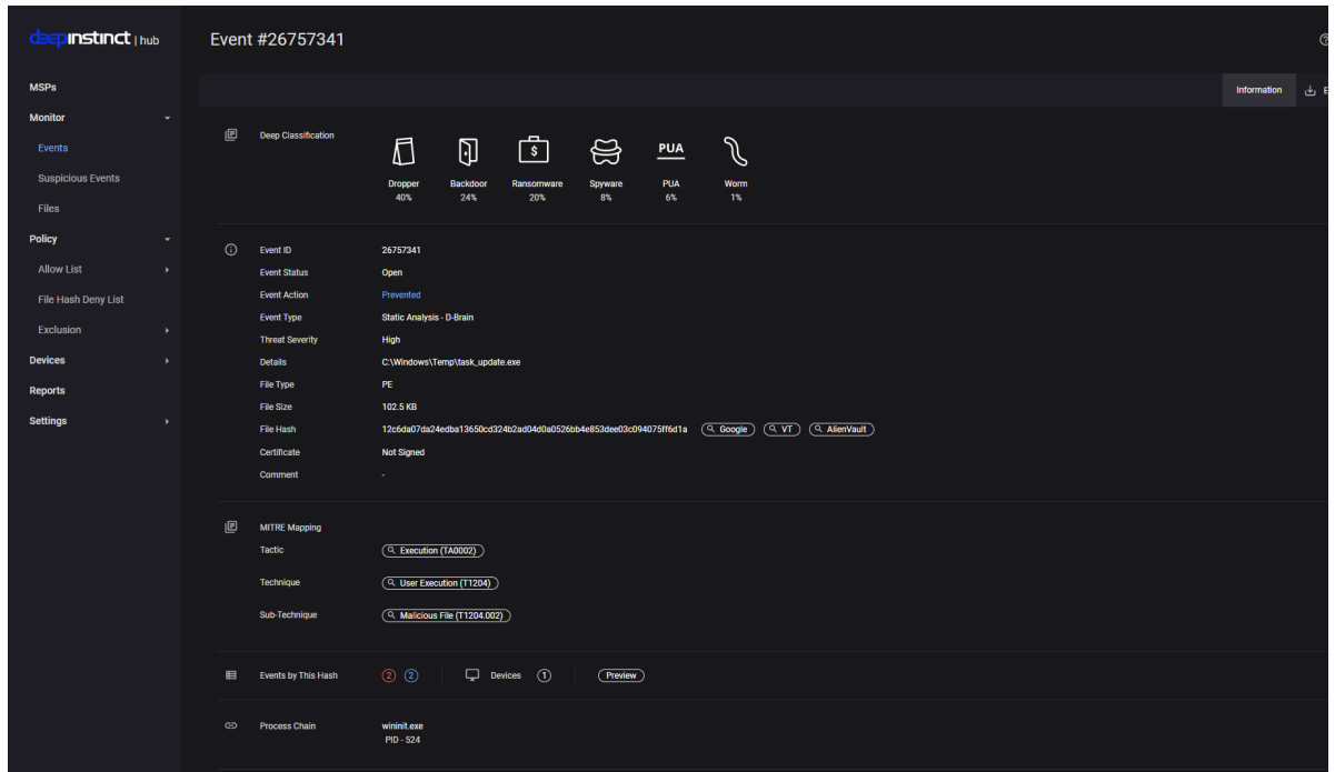
Figure 1: Deep Instinct console showing the prevented event
