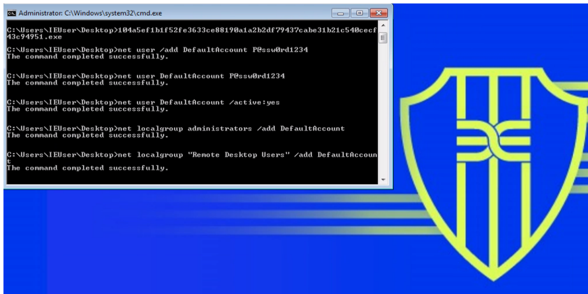
Figure 3: Output from execution of "user.exe"
