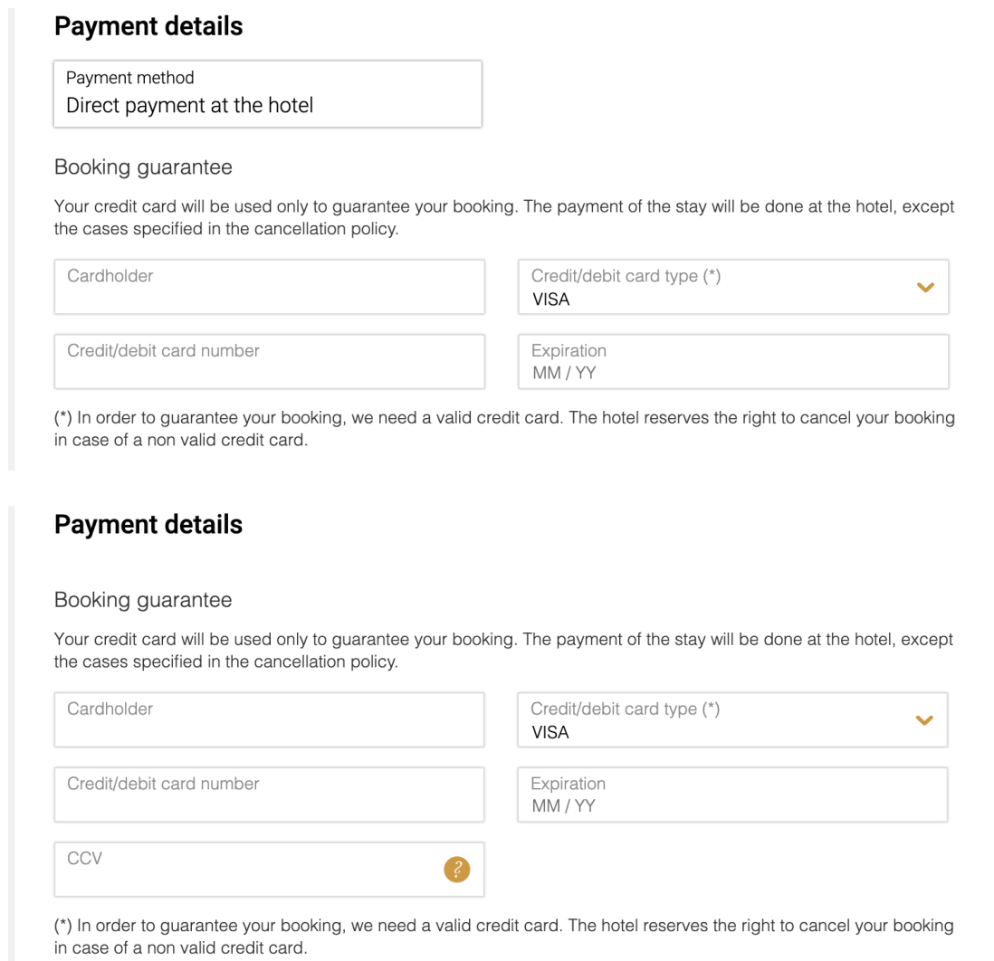
Figure 5. The original credit card form (above) from the hotel website and the injected form (below) from the skimmer
