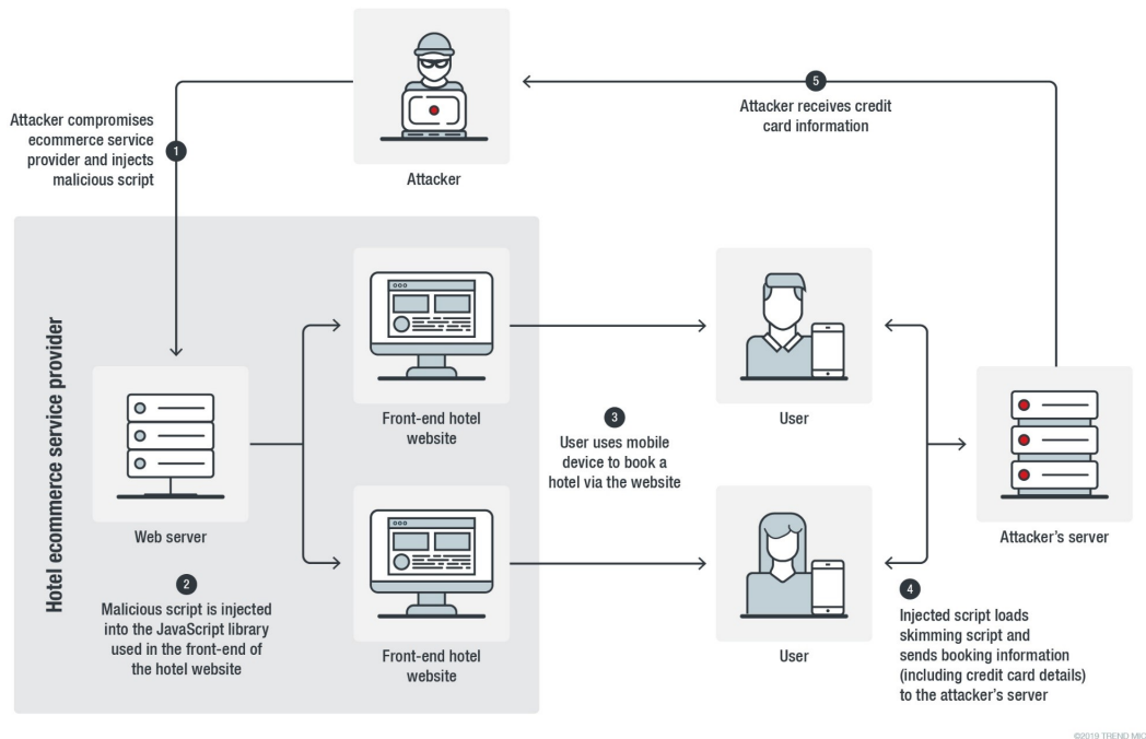
Figure 1. Infection chain of the Magecart skimming attack on the online hotel booking websites
