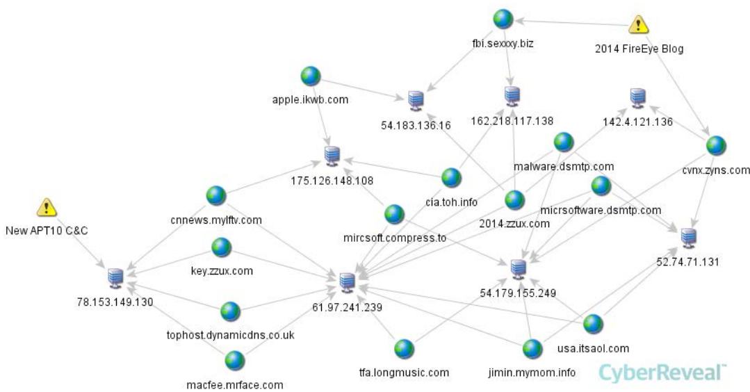
Figure 9: Infrastructure graph linking early Plugx domains to recent APT10 domains
